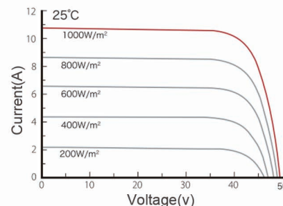
Current-voltage(420W)
