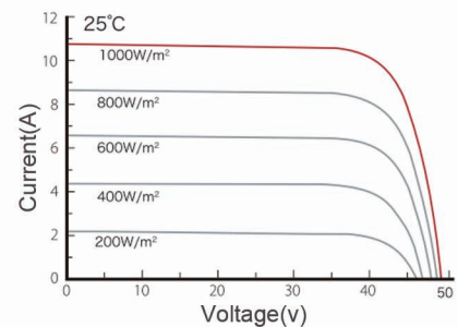
Current-voltage(340W)
