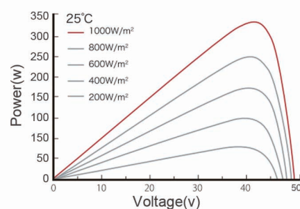
Power-voltage(340W)
